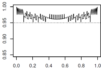
Clopper-Pearson
