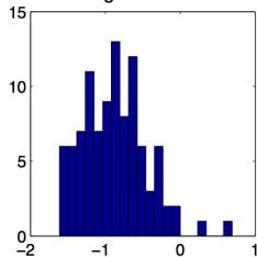
Right skewed
