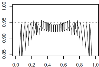
Clopper-Pearson
